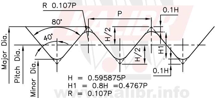
PG THREAD PROFILE
